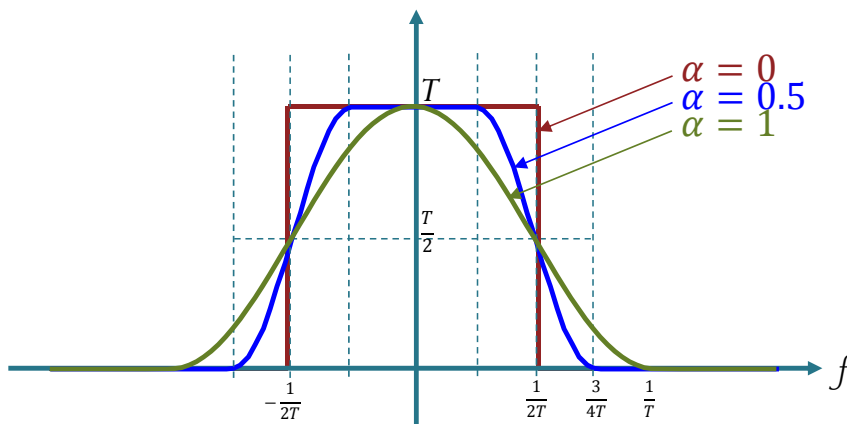
Figure 68: Raised cosine pulse (in the frequency domain) with different values of the roll-off factor
