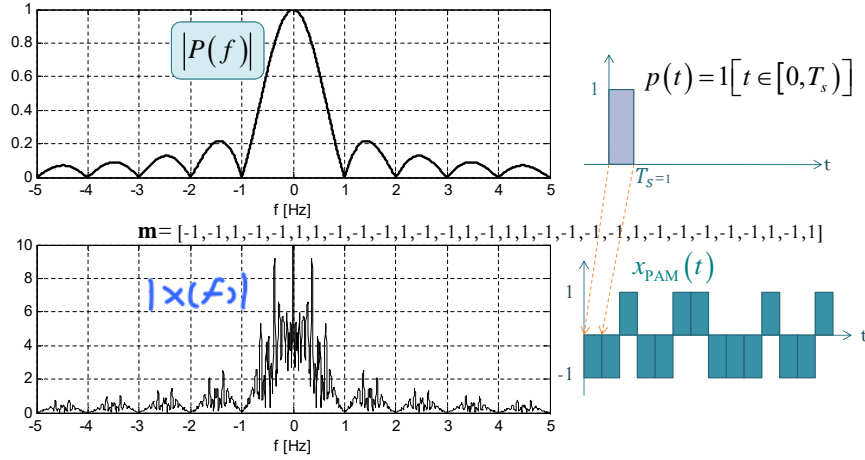
Figure 60: Frequency-Domain Analysis of PAM
