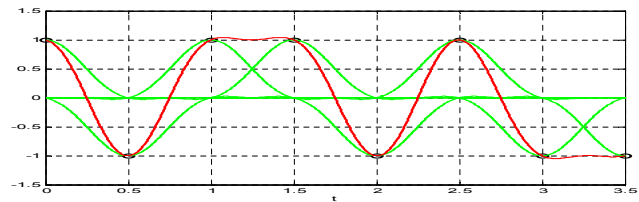
Figure 70: Using the raised cosine pulses in PAM
