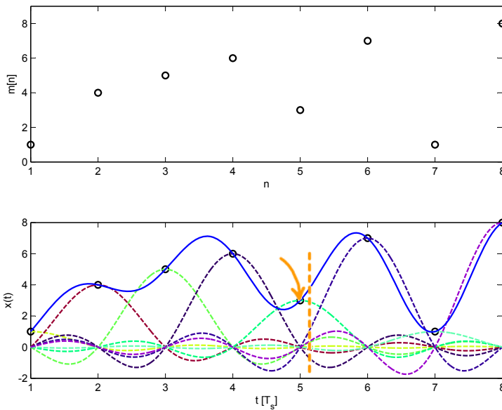
Figure 65: Using the sinc pulse in PAM
