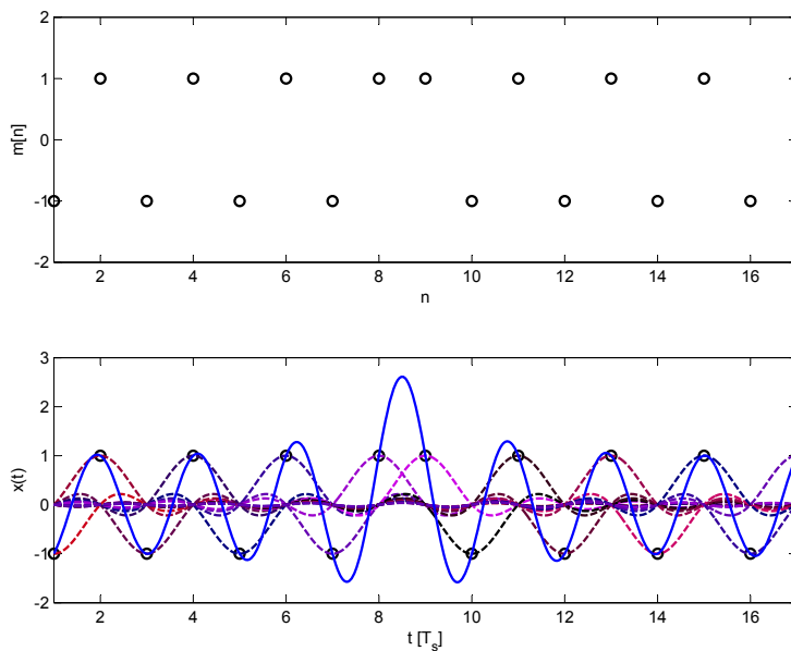
Figure 66: Using the sinc pulse in PAM can cause high peak.
