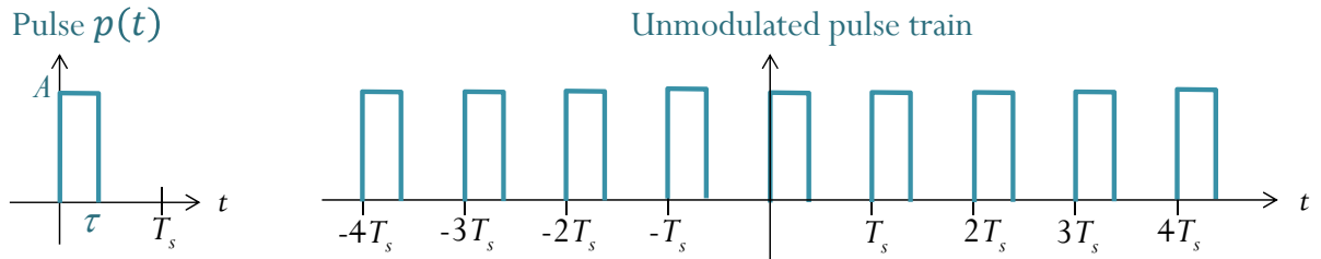
Figure 55: Unmodulated pulse train
