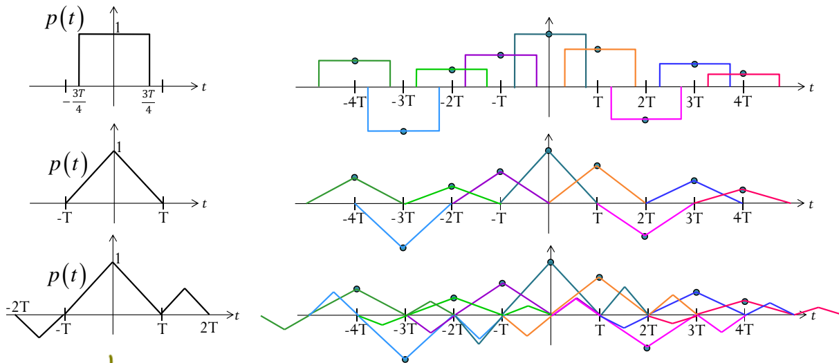
Figure 64: Examples of pulses that do not cause ISI.
