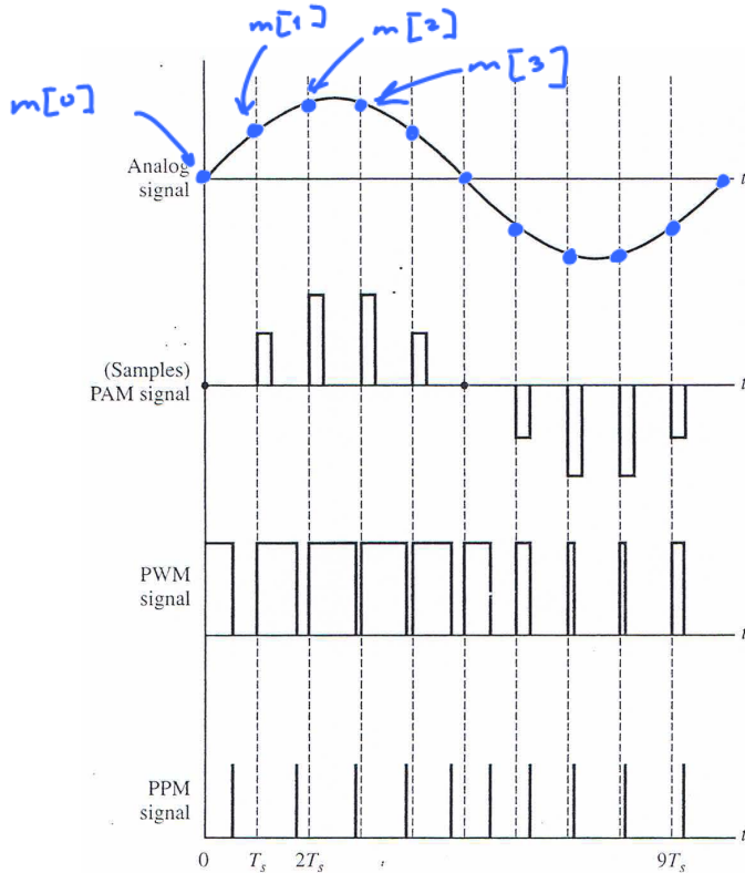
Figure 56: Illustration of PAM, PWM, and PPM. [14, Fig. 3.56]
