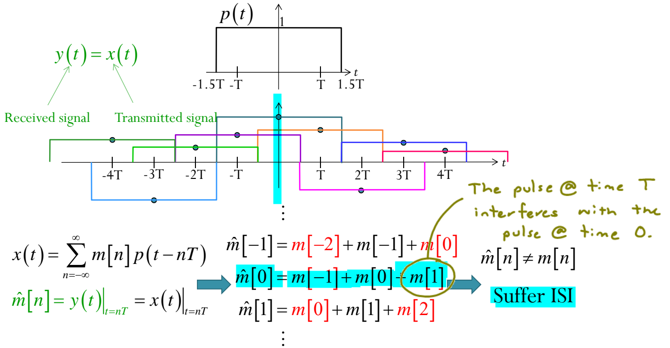
Figure 62: ISI in PAM
