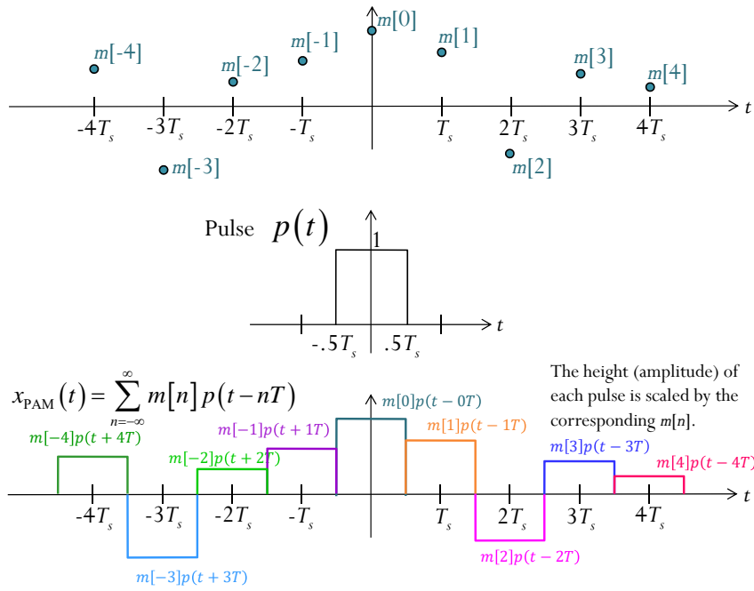
Figure 57: An example of a PAM signal
