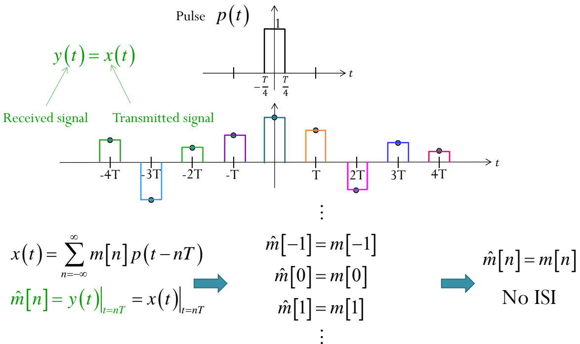
Figure 63: PAM using narrow pulses
