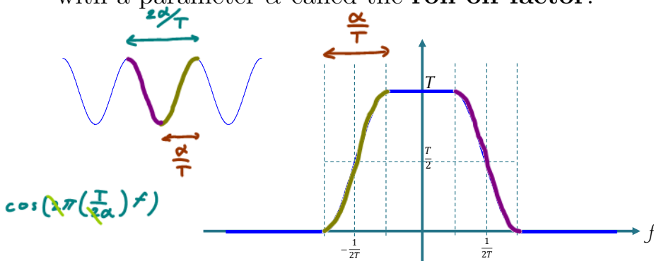
Figure 67: Raised cosine pulse (in the frequency domain)
