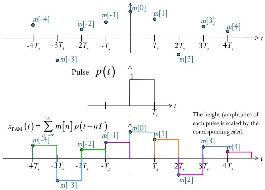
Figure 58: Another Example of a PAM signal
